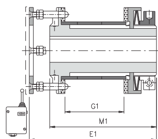
.../SI/ML (long-hub version)
